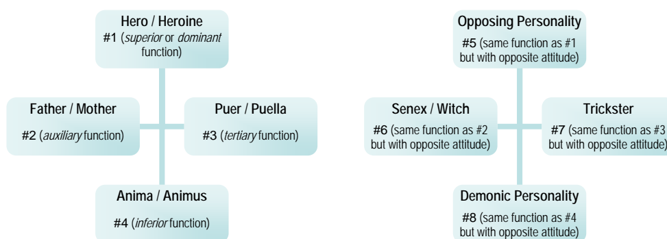
DIAGRAM 1: Archetypal complexes carrying the eight functions of consciousness
